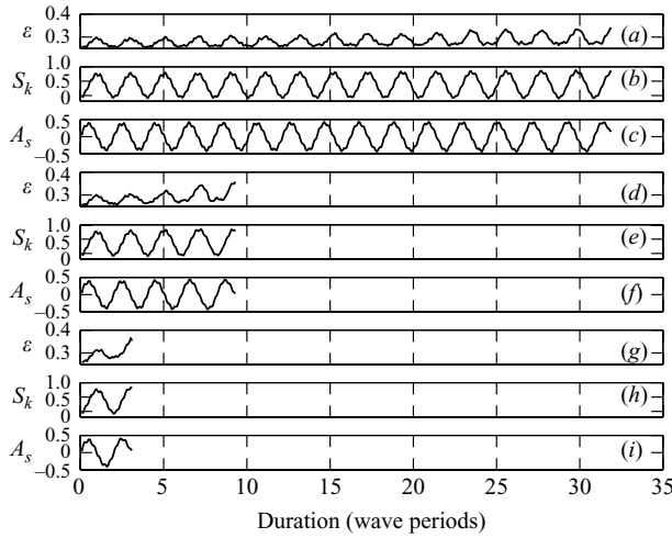
FIGURE 2. Simulations of steepness ( a, d, g ), skewness ( b, e, h ), asymmetry ( c, f, i ) of the wave of IMS = 0.26 as it evolves from the initial conditions to the point of breaking. The values of U/c are 2.5 ( a-c ), 5.0 ( d-f ) and 10.0 ( g-i ). The x -axis shown at the bottom remains the same for all.
