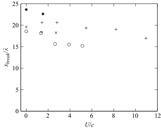
FIGURE 17. Number N of wavelengths to the breaking versus wind forcing U/c : o: IMF = 1.5 Hz; x: IMF = 1.55 Hz; +: IMF = 1.6 Hz; *: IMF = 1.7 Hz.
