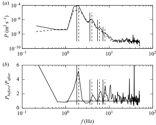
FIGURE 8. (a) Spectra P of the time series of IMF=1.8 Hz, IMS=0.30 , U/c=0 . Solid line corresponds to the pre-breaking spectrum measured at the second probe (see time series in figures 7). Dashed line is post-breaking spectrum measured at the third probe (time series in figure 9). Multiples of IMF are shown with solid vertical lines. Multiples of the incipient breaker 2 Hz frequency are shown with dashed vertical lines. (b) Ratio of the pre-breaking and post-breaking spectra. Solid horizontal line signifies ratio of 1, vertical lines have the same meaning as in (a).
